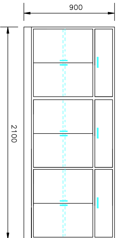
WORKING TABLE/EQUIPMENT BENCH (ITEM No. 8.5)
