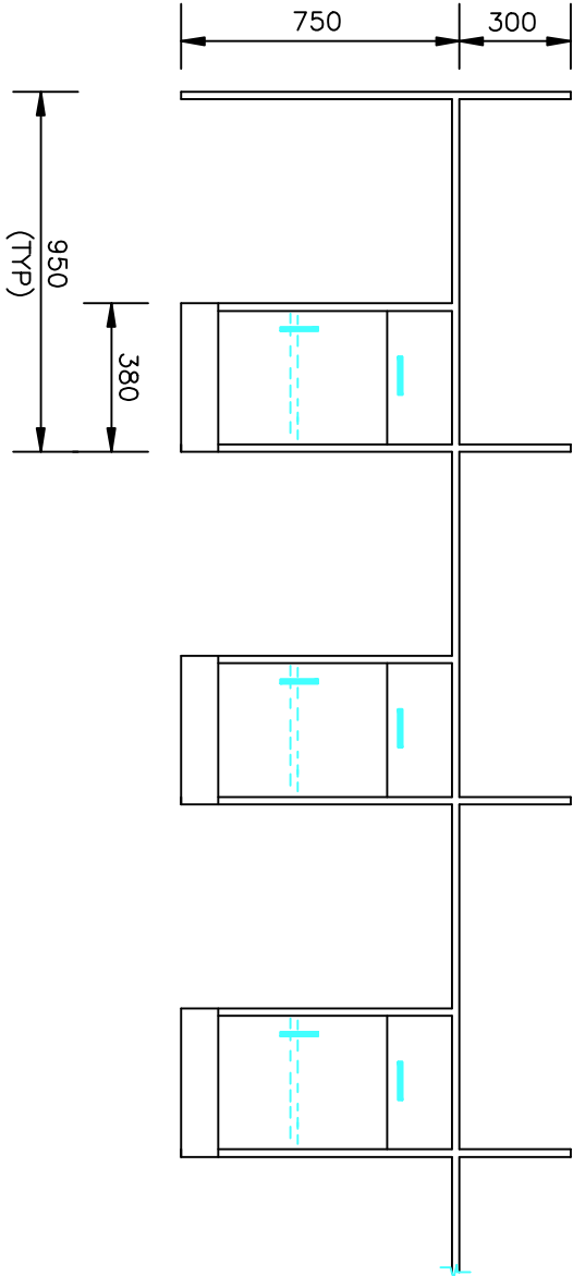
RUNNING TABLE/SITTING TABLE (ITEM No. 8.3)
