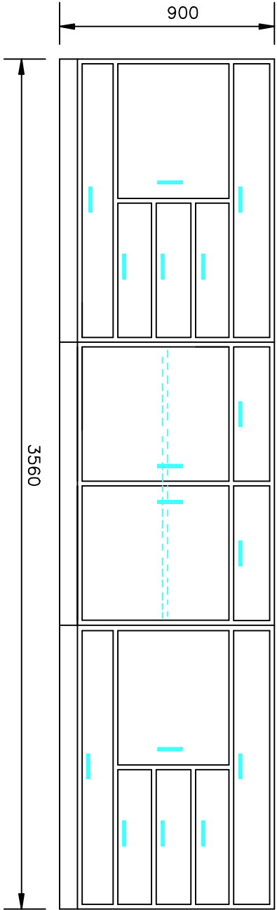
WORKING TABLE/EQUIPMENT BENCH (ITEM No. 8.2 a & b)
