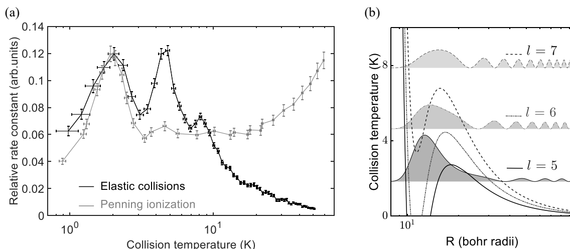
Fig. 1 (a) Relative rate constant of \text{He}^+ \text{-D}_2 elastic collisions with collision energy (black), and Penning ionization process for the same system (gray) [3]. (b) The partial wave \ell = 5 corresponds to the resonance at 2.0 K (below the barrier); the partial waves \ell = 6 and \ell = 7 corresponds to the resonances at 4.0 and 8.0 K (above barrier resonances).
