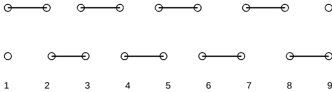
Figure 4. Dimer states in M-G chain
