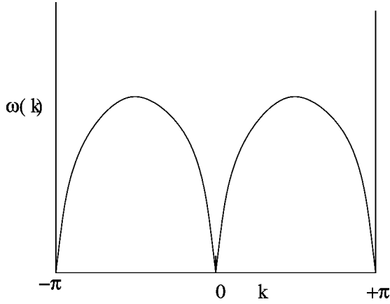
Figure 2. Antiferromagnetic spin waves.
